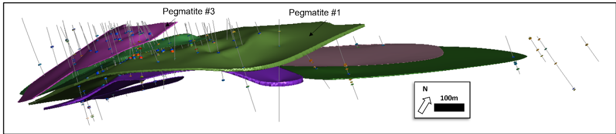
Figure 3: LCT pegmatites within the Raleigh Lake pegmatite field looking west-northwest.
