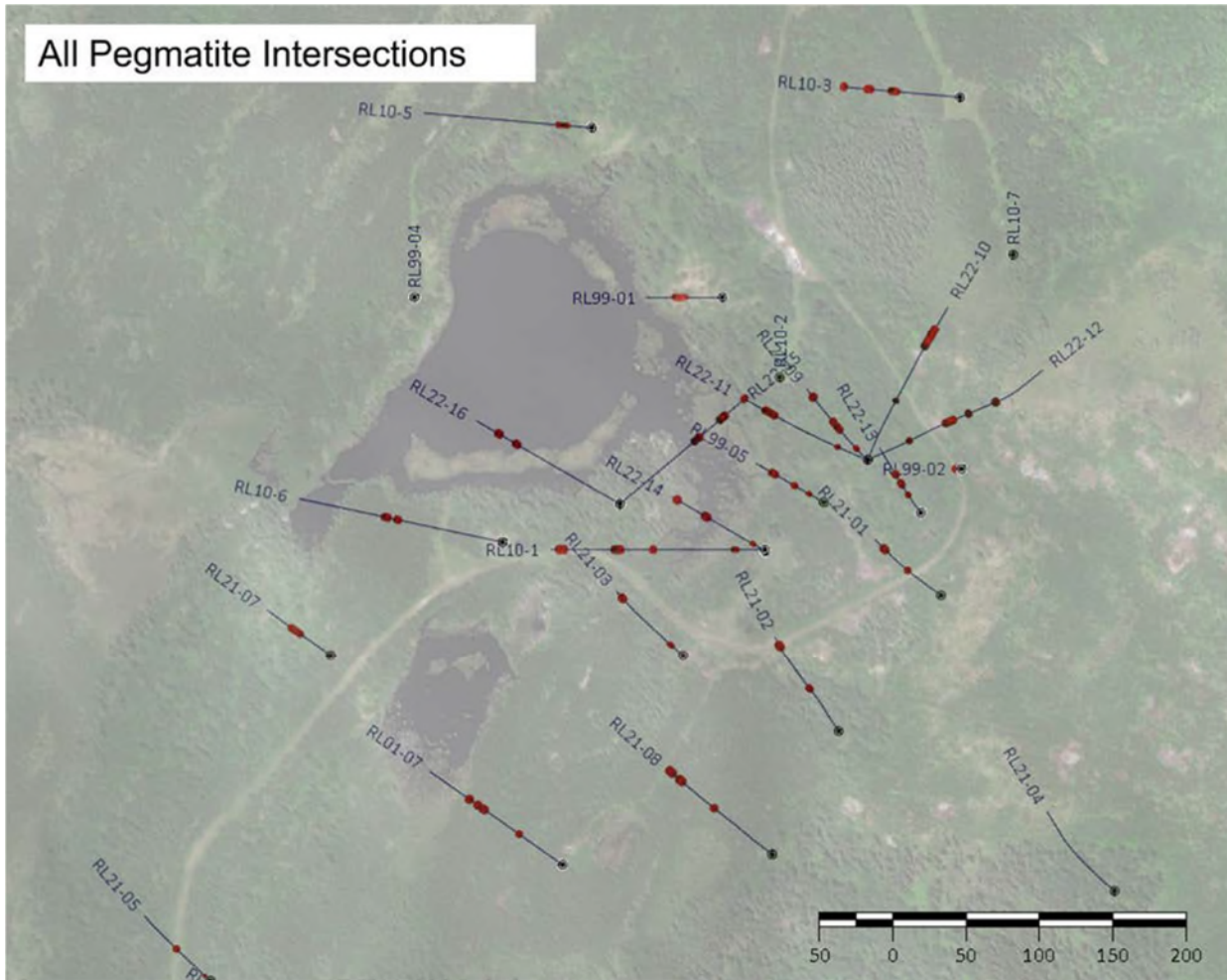
Figure 3: Location of all drill holes in the vicinity of Pegmatite 1 and 3 within Zone 1, highlighting the pegmatite intersections. Note that RL21-04 was terminated prior to intersecting pegmatite. Pegmatite 1 and 3 remain open with depth and additional holes are proposed to test the depth extent during Phase 2 and future drill programs.
